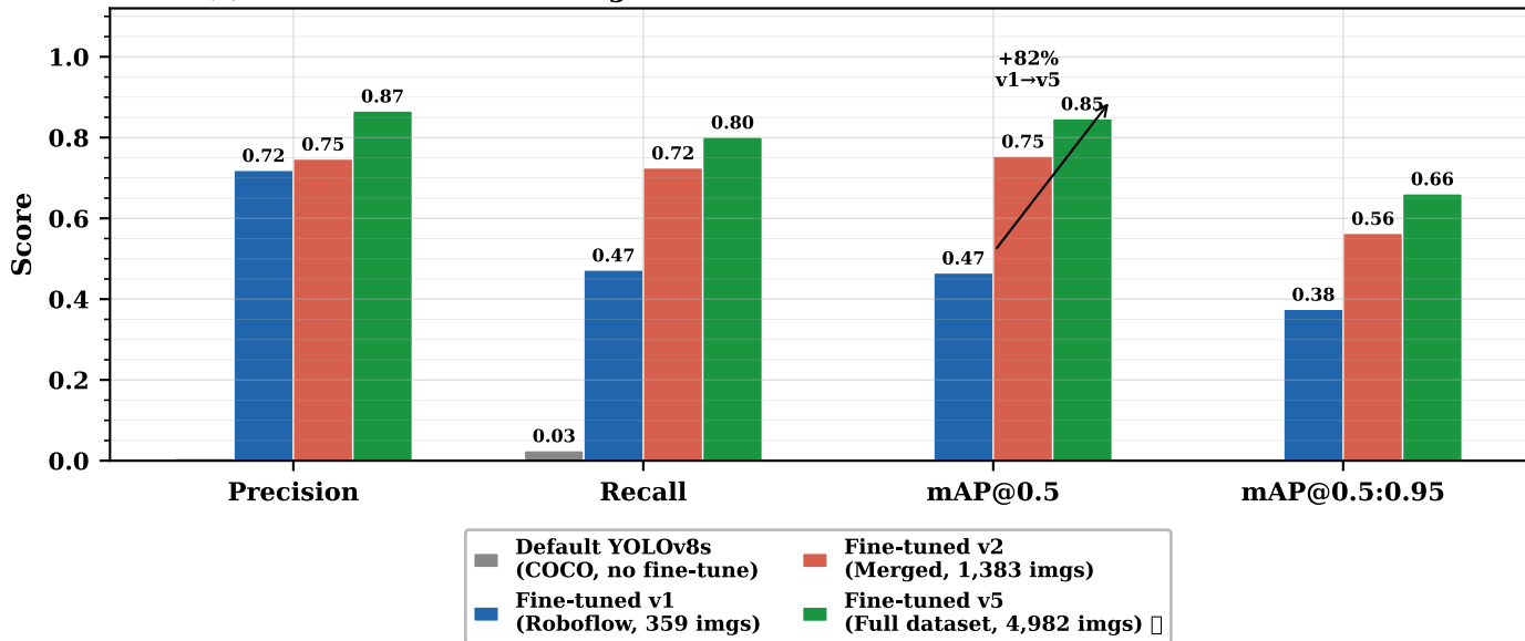
(a) Model Performance Progression on Held-Out Test Set — Default → v1 → v2 → v5
